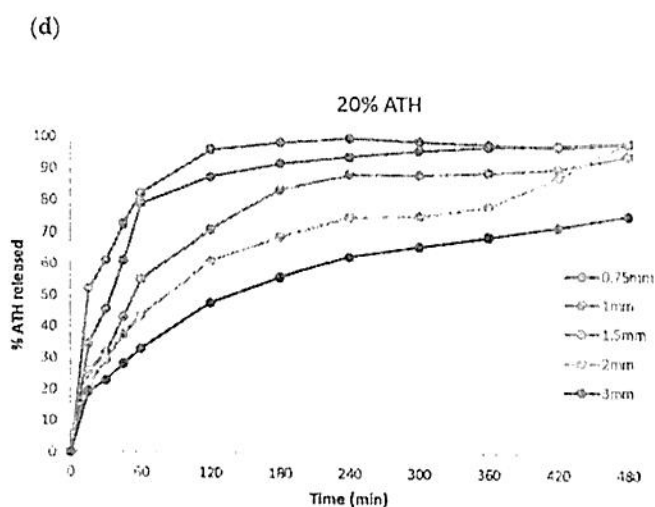
Figure 4. Dissolution profiles of fabricated tablets containing: (a) 5%; (b) 10%; (c) 15%; and (d) 20% of ATH.
