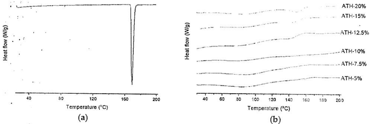
Figure 5. DSC (differential scanning calorimetry) thermograms of: (a) pure ATH prior to printing, and (b) the DLP 3D-printed tablets with different amounts of ATH.
